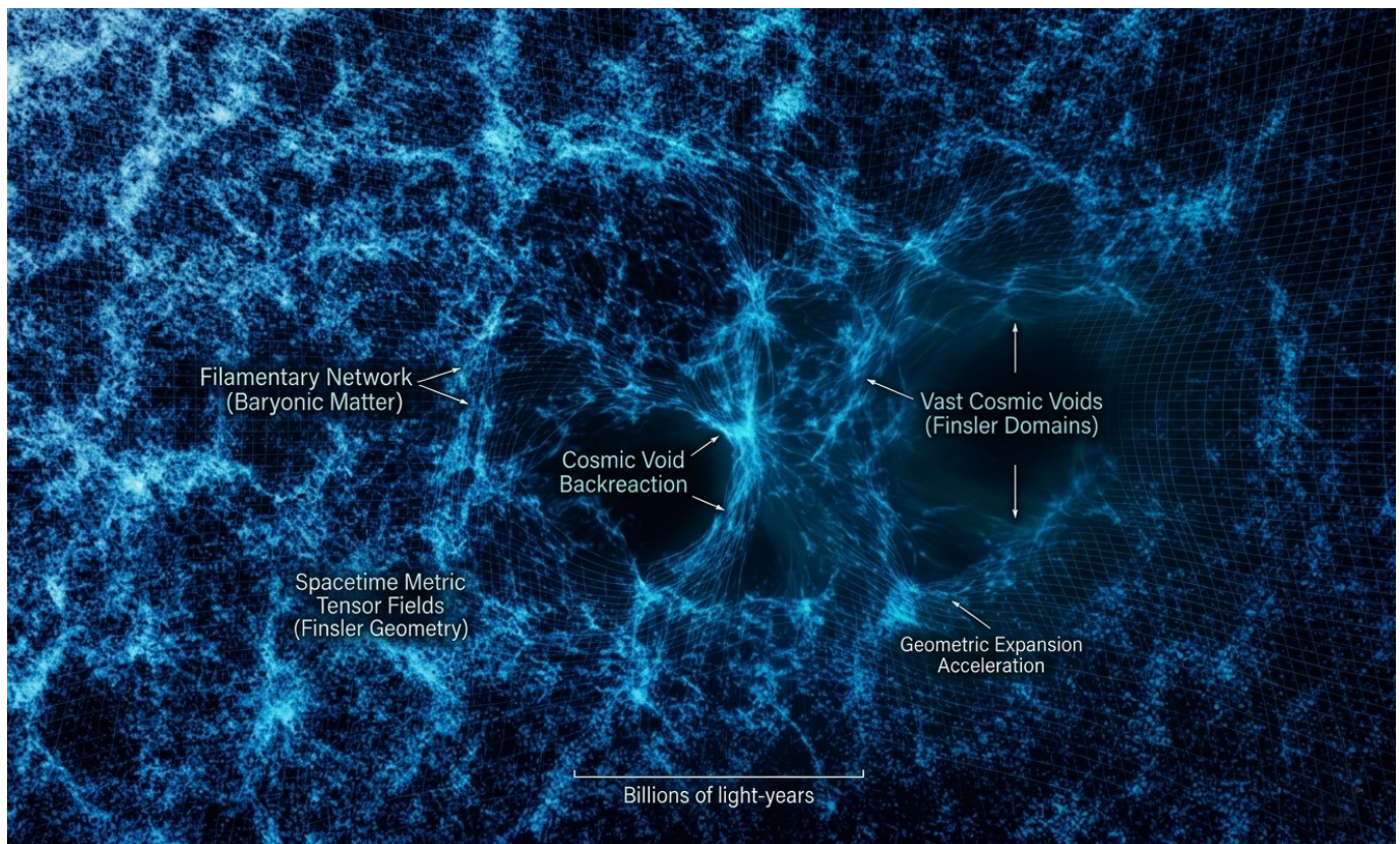
Figure 1 – DESI 3D
